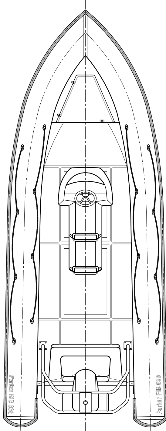
PLAN VIEW
